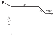
I Double Angle TLDA7 10'2"
