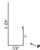
P Universal Sidewall TLUS8 10'2"
