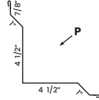
G Residential Eave TLRE35 10'2"
