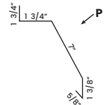
T Track Cover Cannonball FM TLCT15 10'2"
