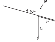
K Post Trim TLPT10 10'2"
