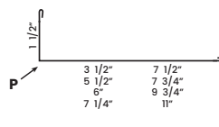
O Notched Endwall / Everlast II® Profile TLNEEL32 42"
