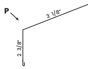
J Drip Cap TLDC9 10'2"
